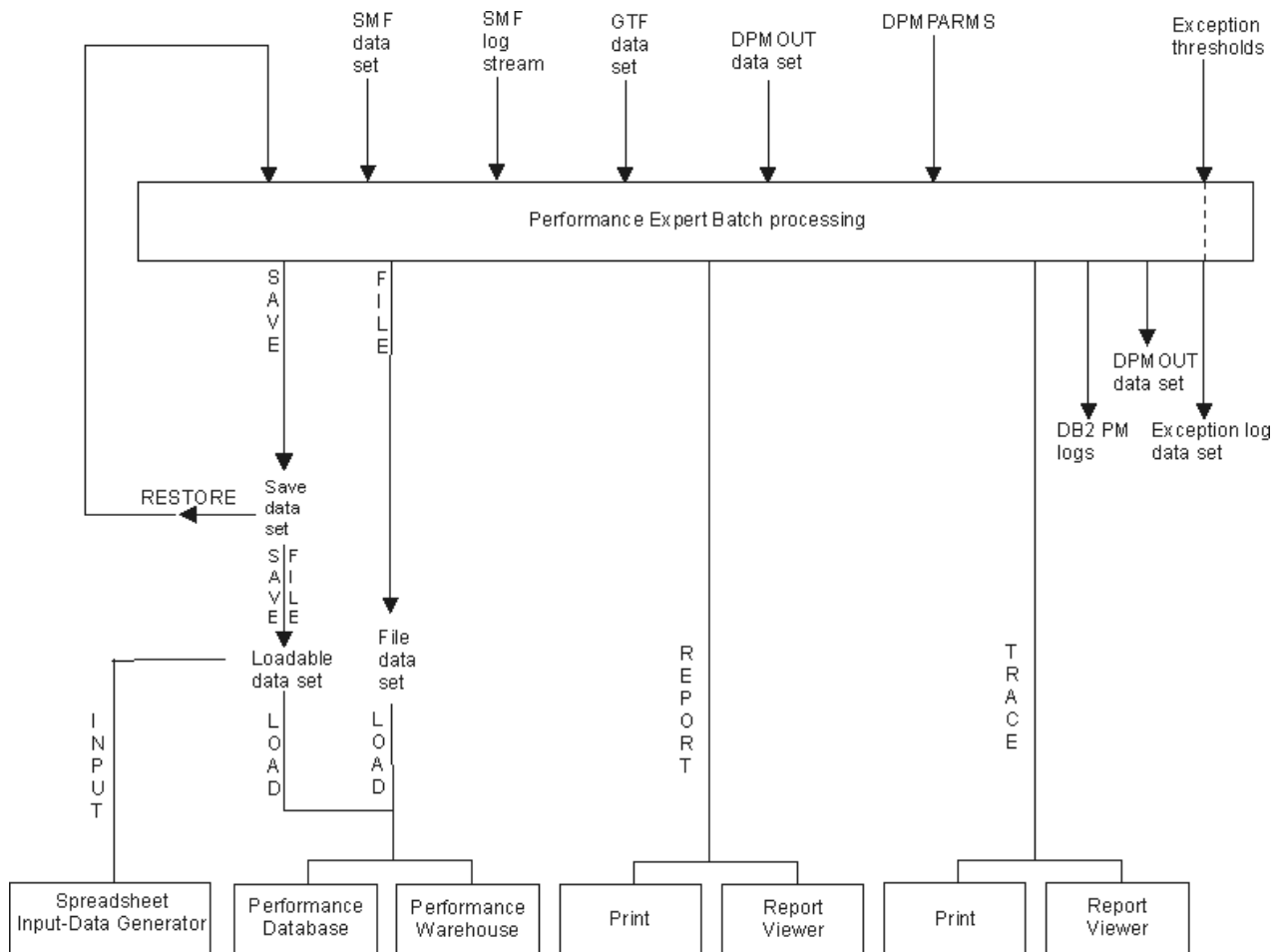
Figure 2. OMEGAMON XE for DB2 PE reporting
